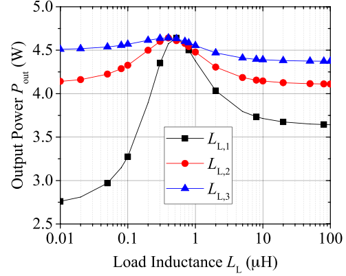
Figure 6. Simulated output power P_{out} as function of varying load inductance for the analyzed numerical example. One of the three load inductances is varied while keeping the other two fixed at their optimal value.
