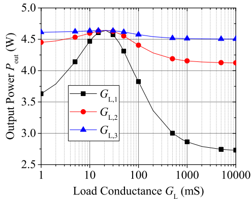
Figure 5. Simulated output power P_{out} as function of varying load conductance for the analyzed numerical example. One of the three load conductances is varied while keeping the other two fixed at their optimal value.
