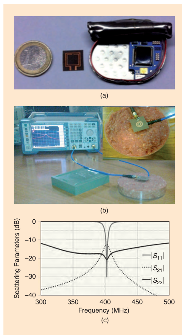
Figure 18. The WPT link for implantable pacemakers proposed in [59]. (a) A photo comparing the receiver of the WPT link proposed in [59] and a single-chamber non-rate-responsive Discovery II pacemaker (model 481) by Guidant. (b) The experimental setup adopted for scattering-parameter measurements. (c) The measured scattering parameters.
