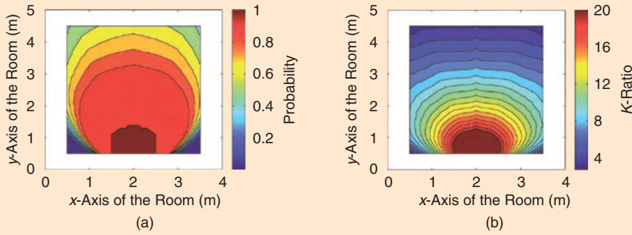
Figure 14. The characteristic result of the probabilistic model in [44]. (a) The probability of reception x polarization and (b) the Rician distribution K ratio (dB) for x-polarized tags.
