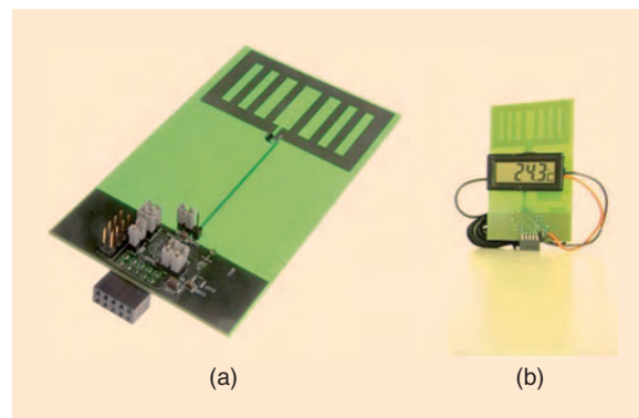
Figure 10. A printed circuit board (PCB)-integrated rectenna and its power management: (a) the PCB and (b) the system powering a temperature sensor with display.
