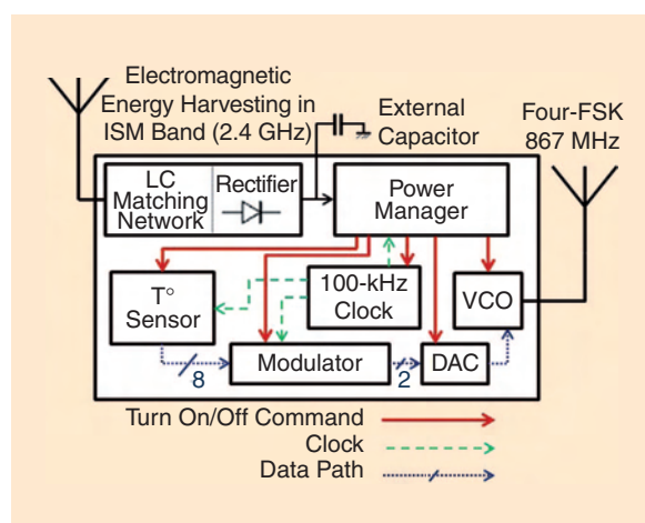
Figure 51. A wireless and batteryless temperature sensor architecture.
