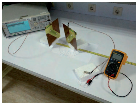
Figure 26. The prototype used in the experimental validation of REC.
