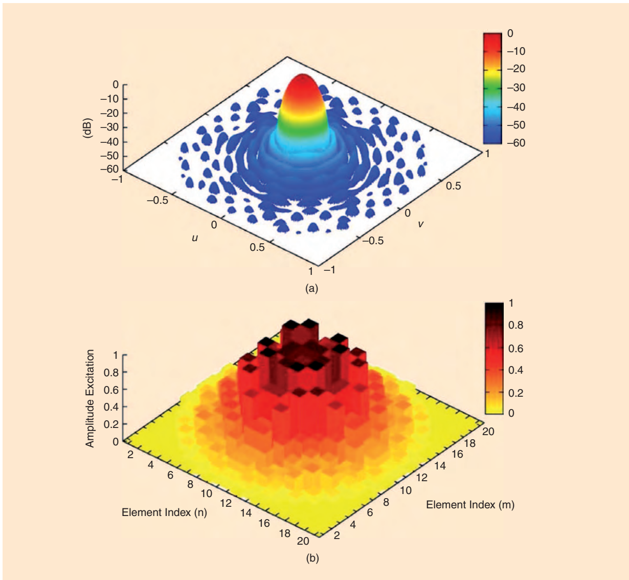
Figure 13. The (a) power pattern and (b) distribution of the amplitude weighting coefficients of an optimal Slepian planar array.
