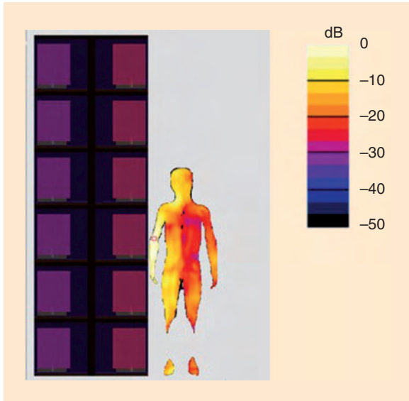
Figure 49. The Ionian standing sideways 5 mm away from the edge of the shelf when all shelf antennas are radiating. The maximum SAR value is identified at the arm.
