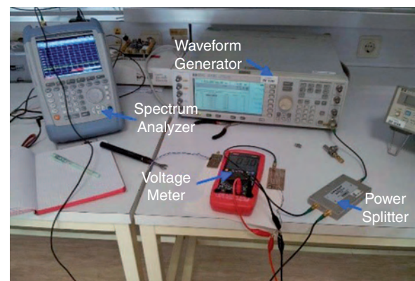
Figure 3. The measurement configuration for the tests described in the “Modeling Aspects of RF–dc Conversion” section.
