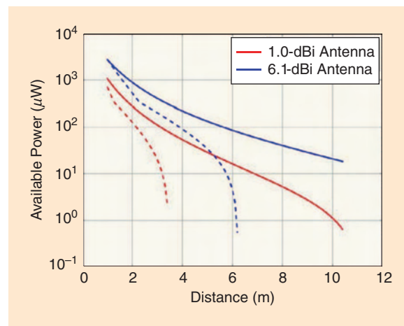
Figure 9. The average obtained dc power versus free line-of-sight distance for two antennas. The solid lines represent the results for the circuit described in Figure 6. The dashed lines represent the results for a commercially available radiative WPT system tested for the same EIRP but for a frequency of 915 MHz.
