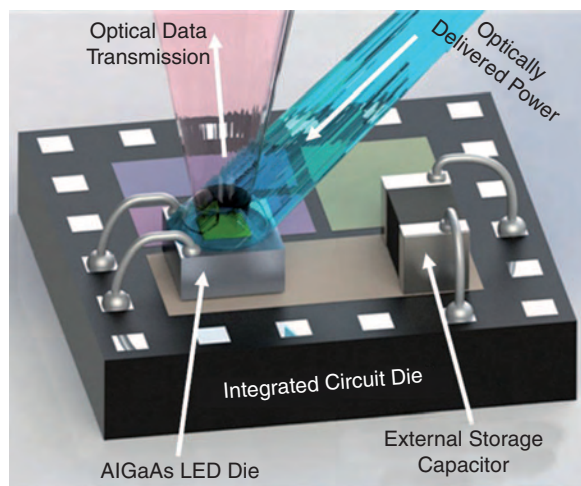
Figure 50. A conceptual representation of an optically powered and optically transmitting microsystem using a single LED.
